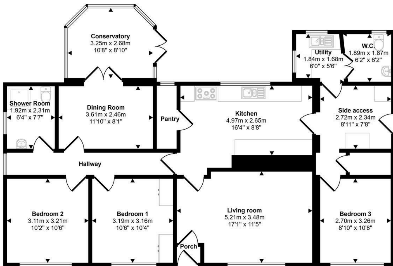
Floorplan
